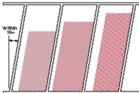
RACKING SYSTEM
